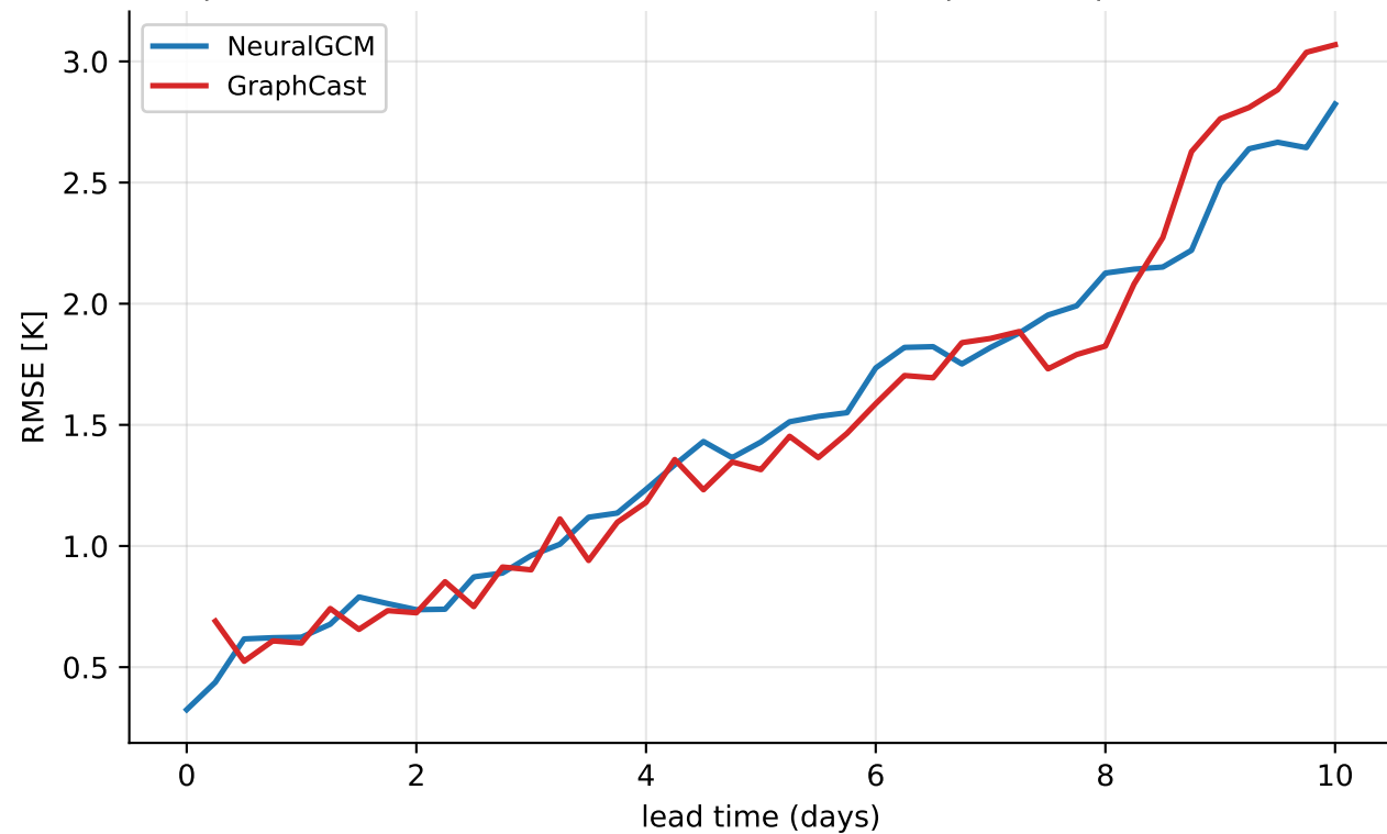
Europe heat-wave 2023-07-28..2023-08-04 — footprint temperature@850 hPa (mean of 18 rollouts)
