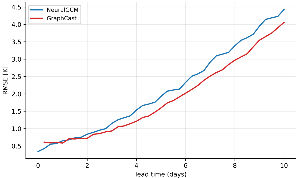
temperature@850 hPa — mean RMSE over all cordex heat waves (9 events, > p99)
