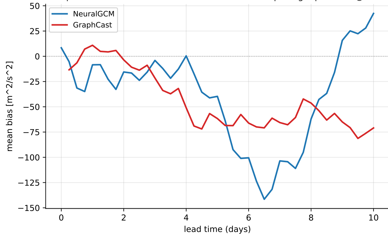
Europe heat-wave 2023-06-25..2023-06-29 — footprint geopotential@500 hPa (mean of 15 rollouts)
