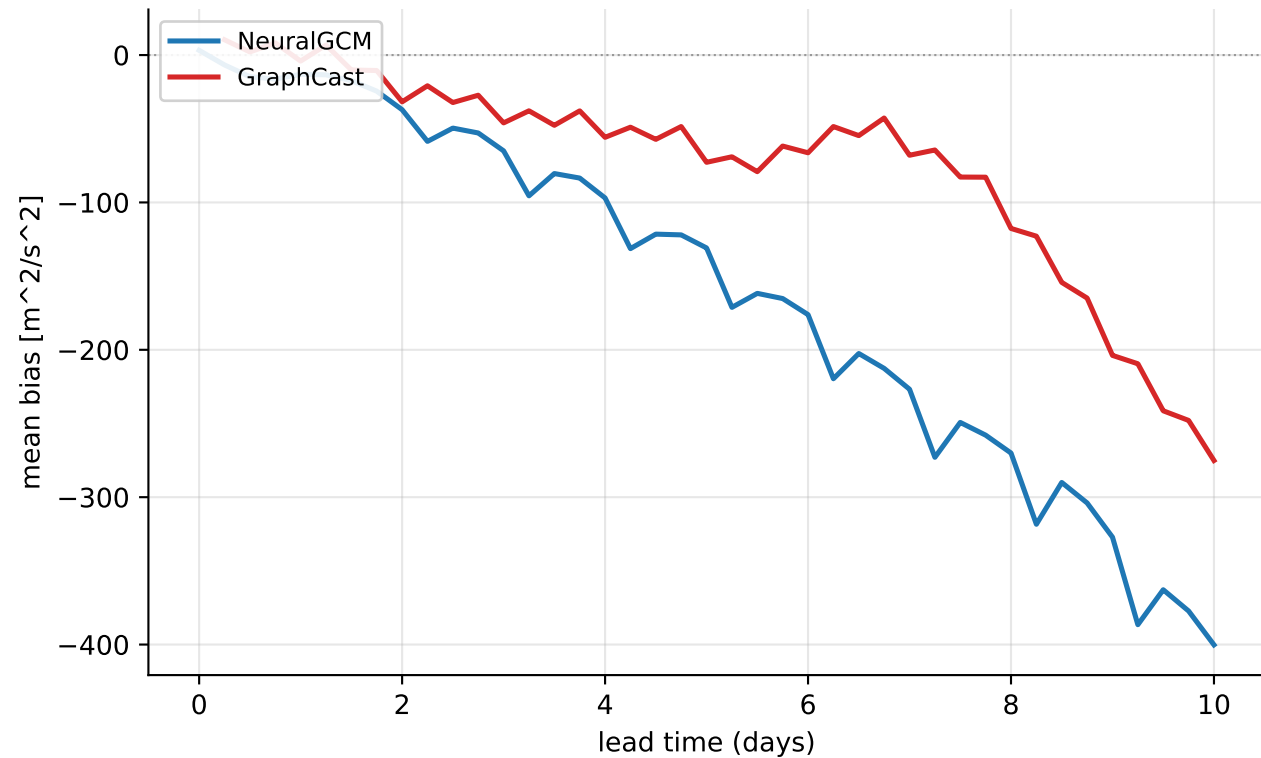
Europe heat-wave 2026-07-09..2026-07-24 — footprint geopotential@500 hPa (mean of 14 rollouts)
