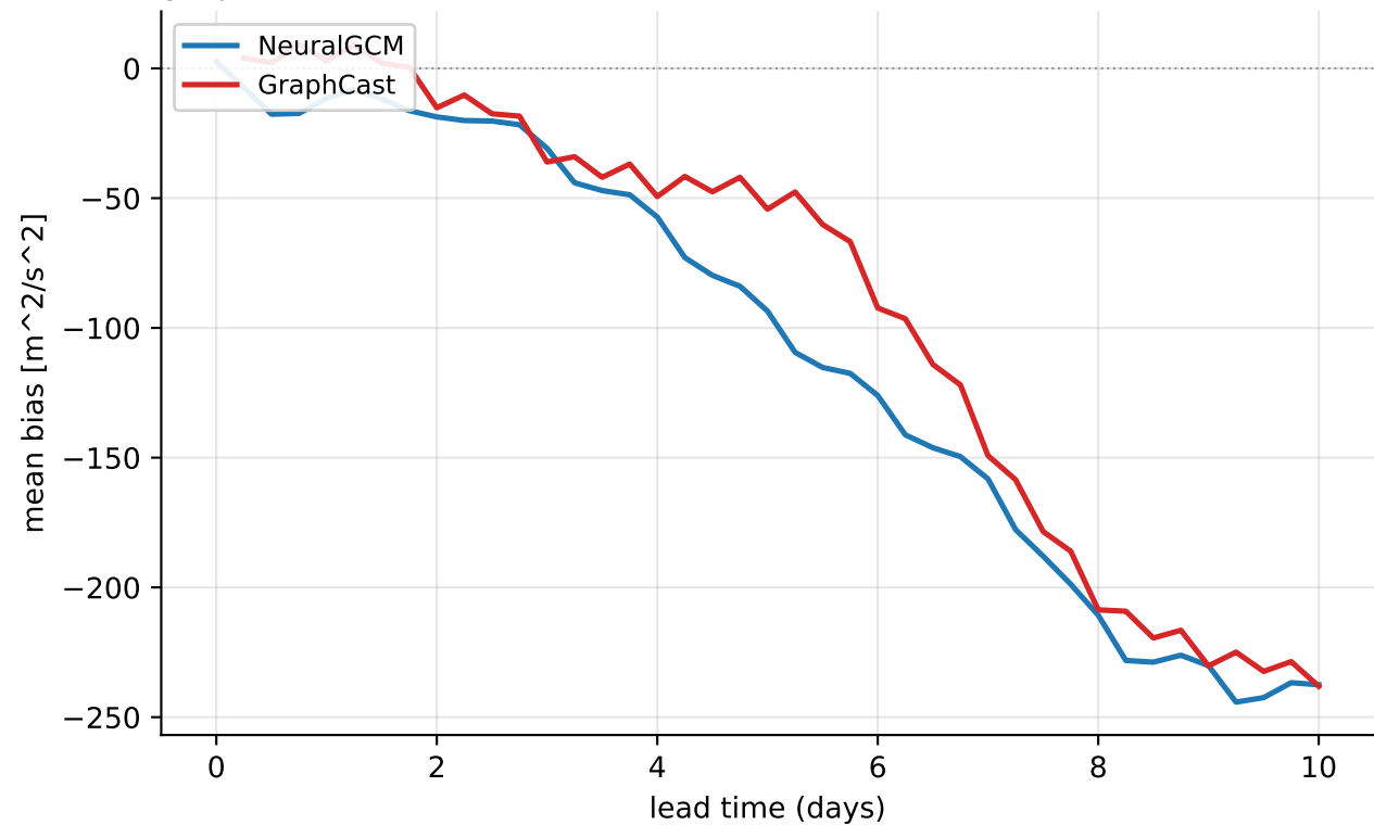
geopotential@500 hPa — mean bias over all mixture heat waves (16 events, > p99)
