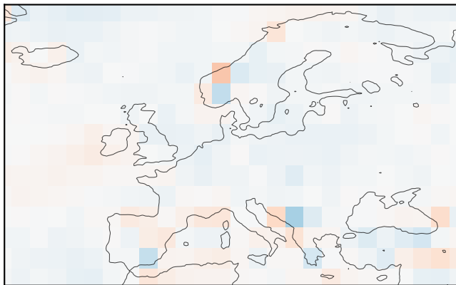
GraphCast
