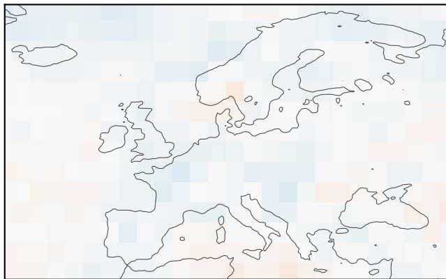
NeuralGCM
