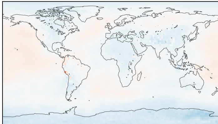
NeuralGCM
