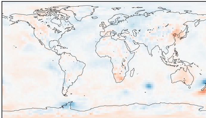
NeuralGCM
