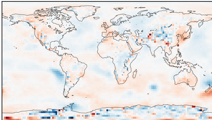
GraphCast
