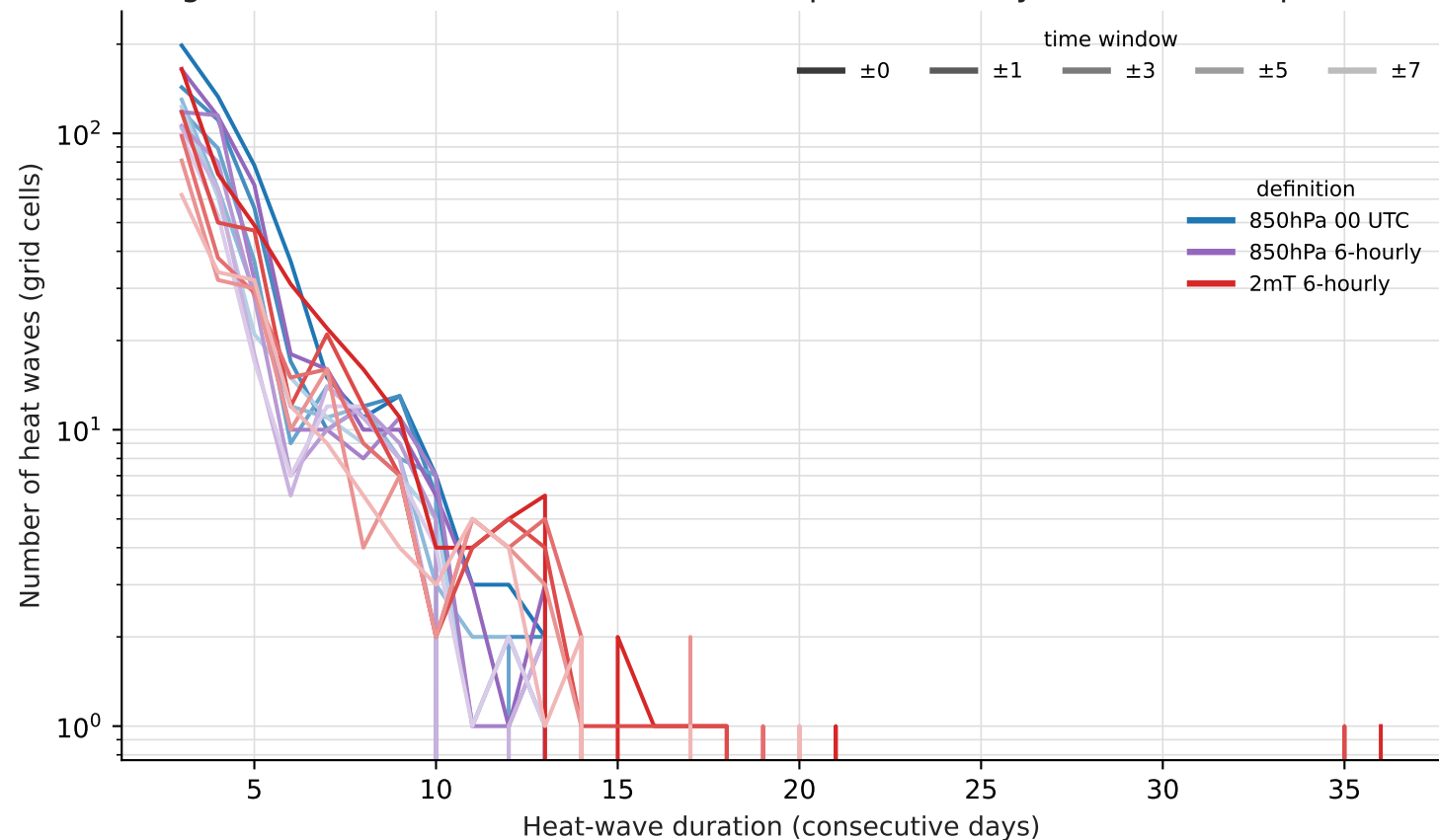
Length of heat wave classification in Europe in 2026 by definitions (> p99)
