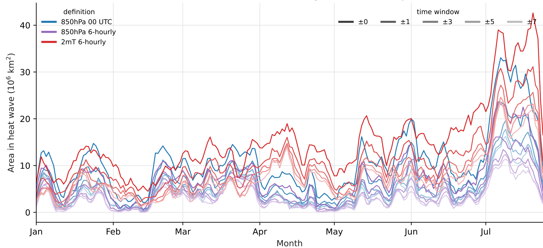
Area classified as heat wave in the world in 2026 by definitions ( > p99 )
