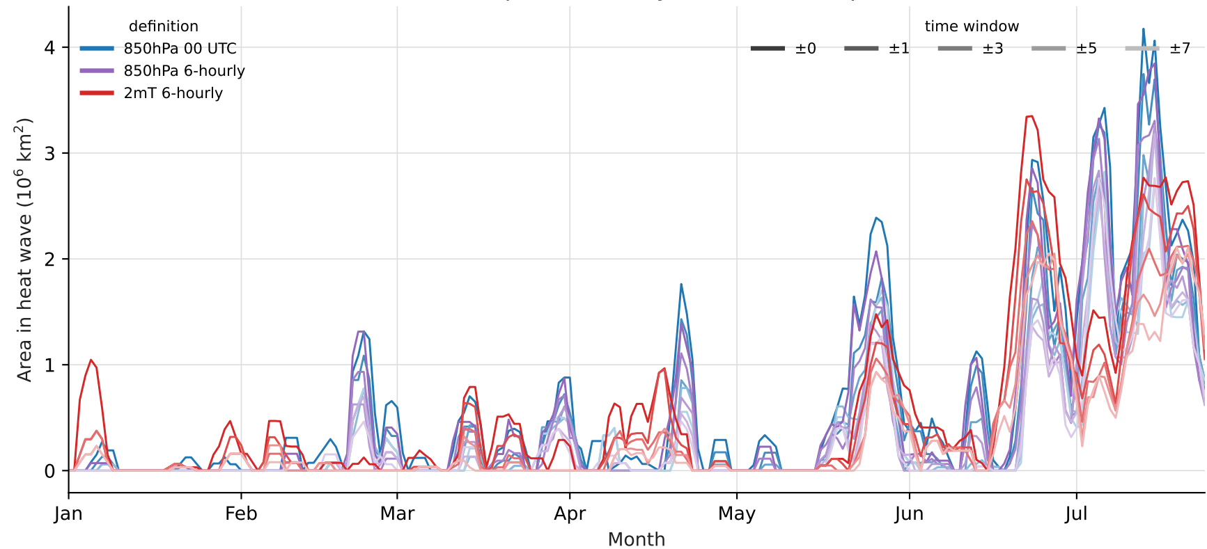
Area classified as heat wave in Europe in 2026 by definitions ( > p99 )
