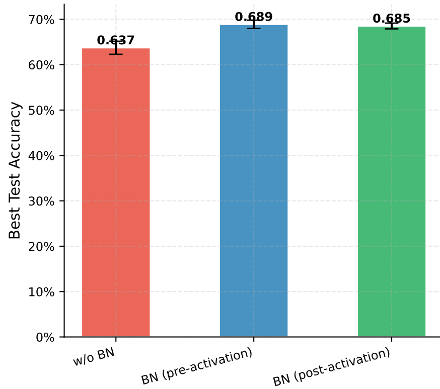
(b) Final Accuracy
