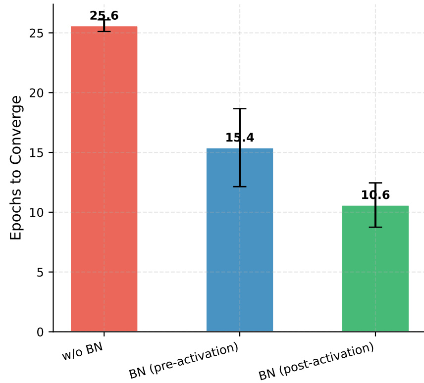
(a) Convergence Speed
