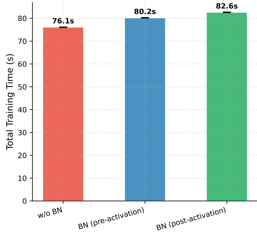
(c) Training Time
