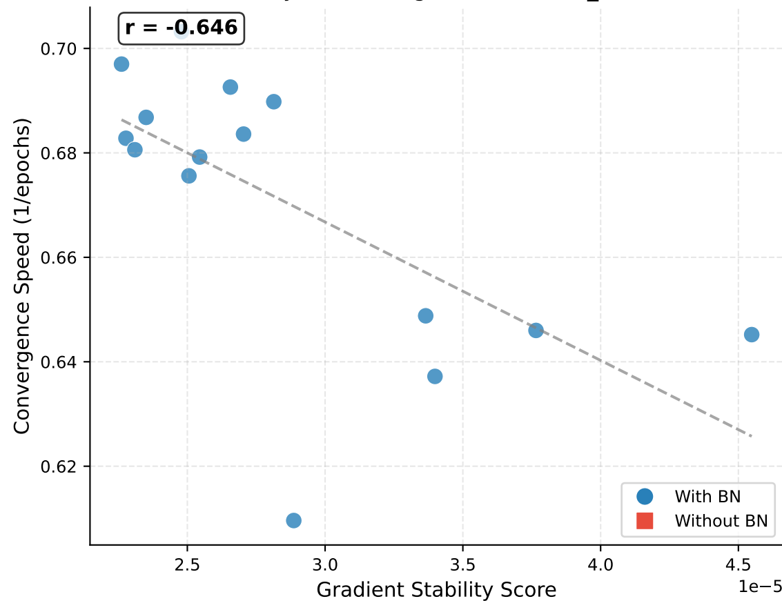
(a) Stability vs Convergence (CIFAR10_resnet18)
