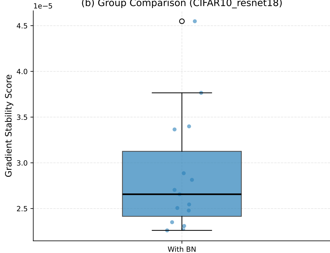
(b) Group Comparison (CIFAR10_resnet18)
