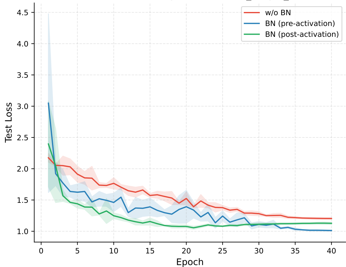
(b) Test Loss Convergence (CIFAR10_simple_cnn)
