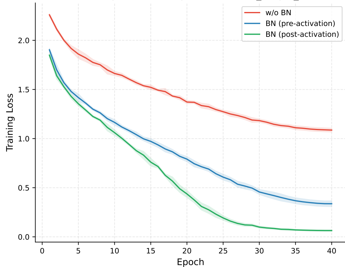
(a) Training Loss Convergence (CIFAR10_simple_cnn)
