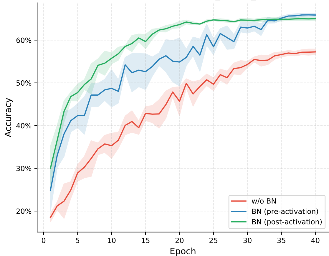
(b) Test Accuracy (CIFAR10_simple_cnn)
