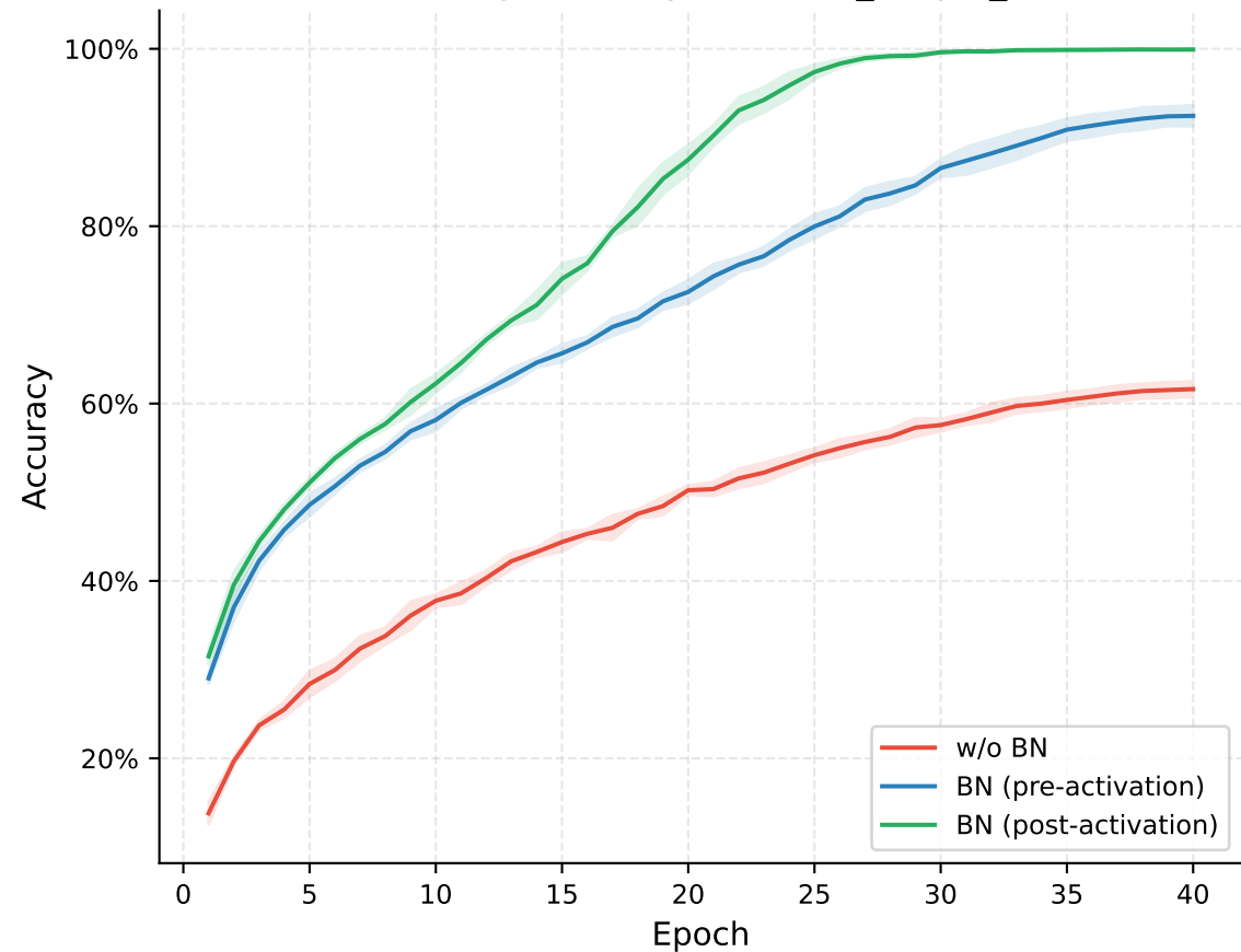
(a) Training Accuracy (CIFAR10_simple_cnn)
