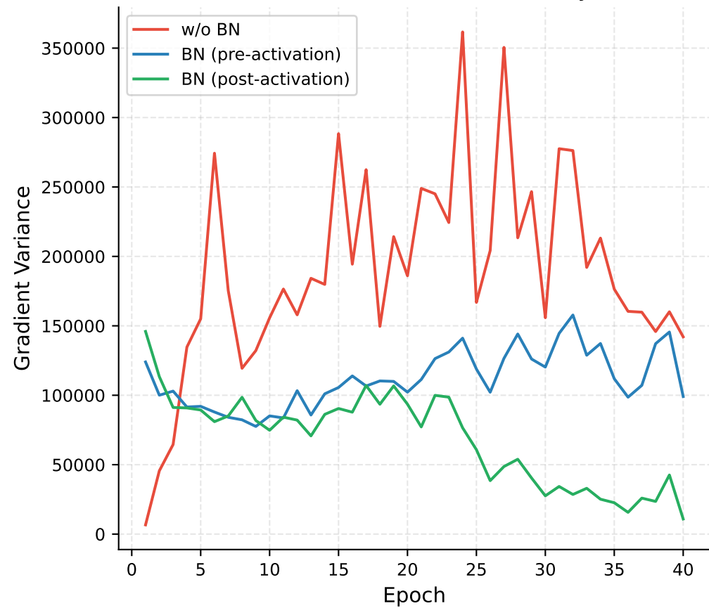
(c) Gradient Variance Evolution (Layer 2)
