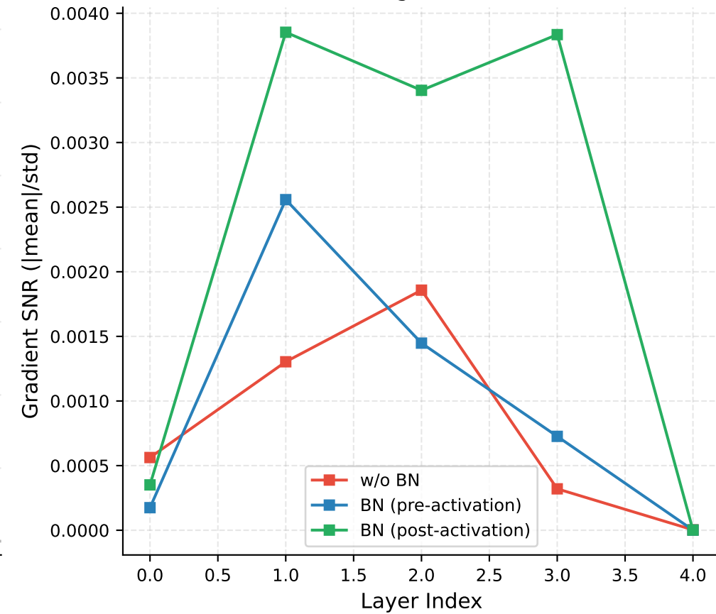
(e) Gradient Signal-to-Noise Ratio
