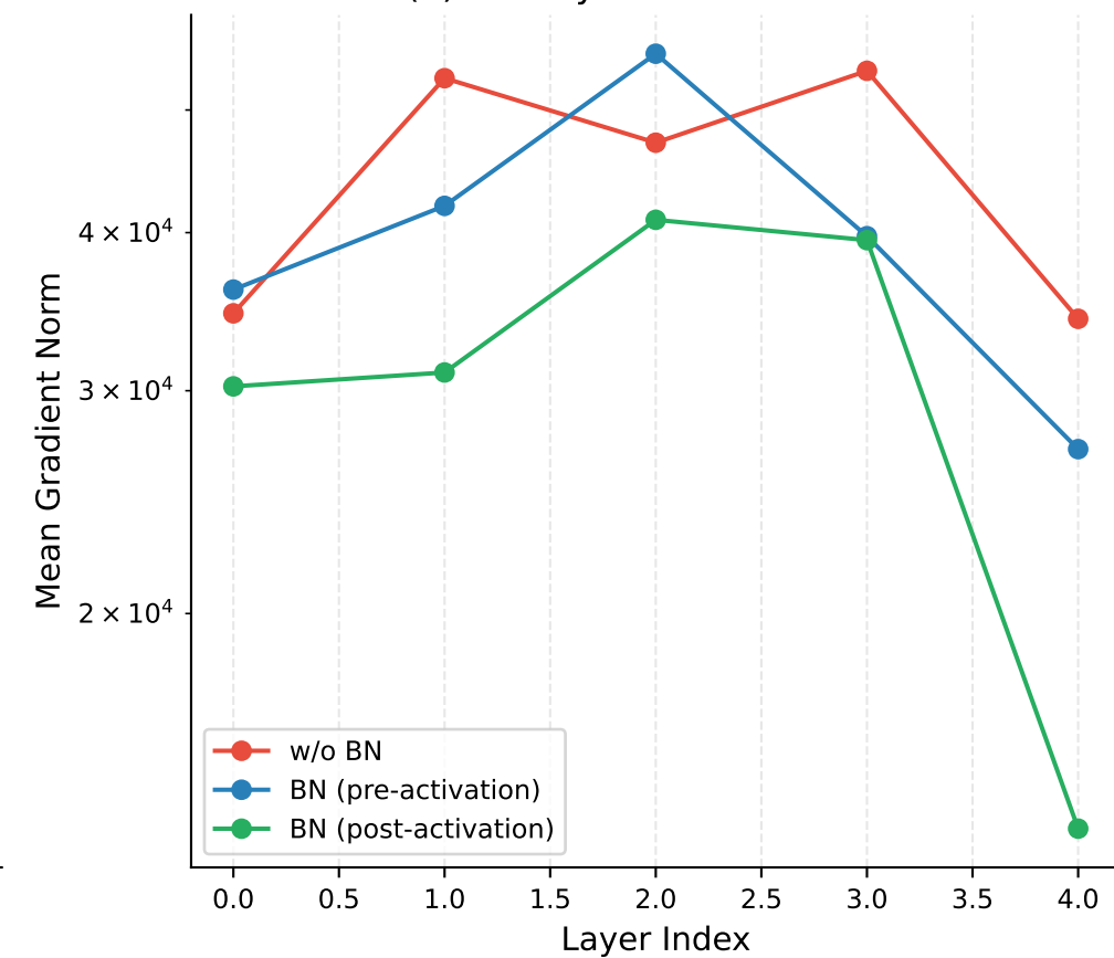
(b) Per-Layer Gradient Norm
