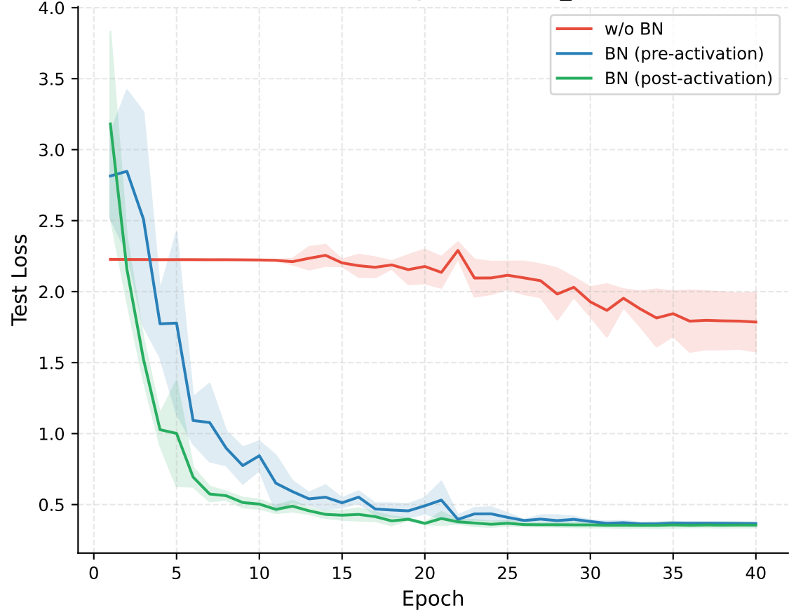
(b) Test Loss Convergence (SVHN_resnet18)
