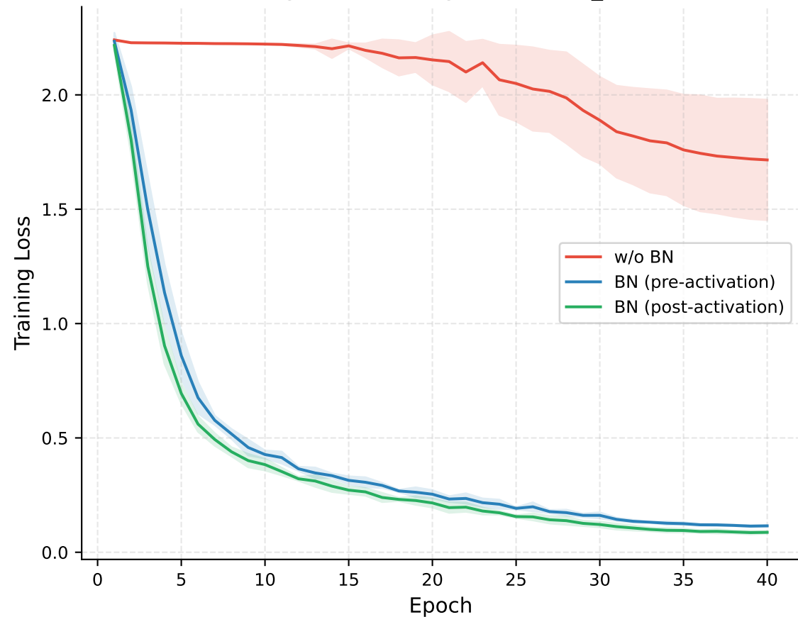
(a) Training Loss Convergence (SVHN_resnet18)
