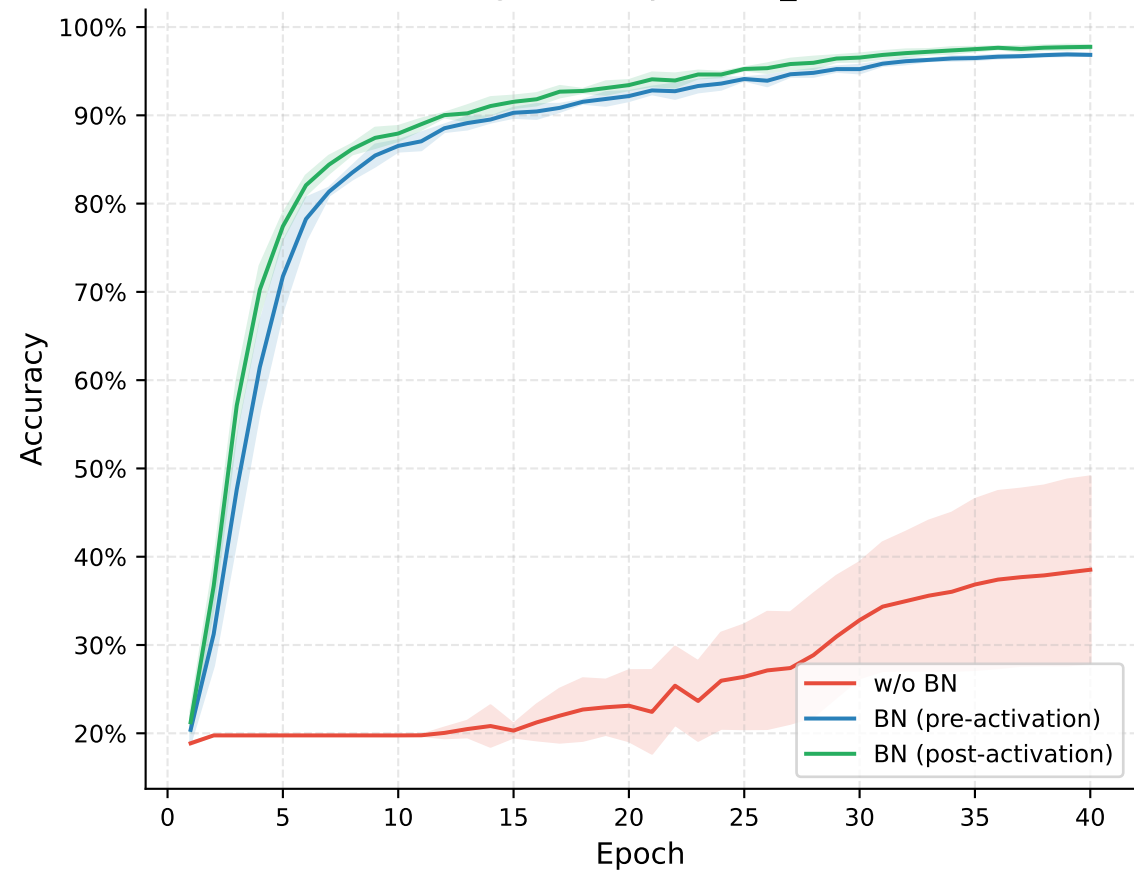
(a) Training Accuracy (SVHN_resnet18)
