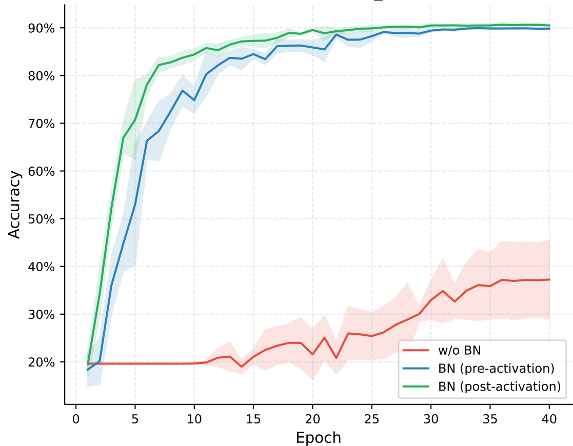
(b) Test Accuracy (SVHN_resnet18)
