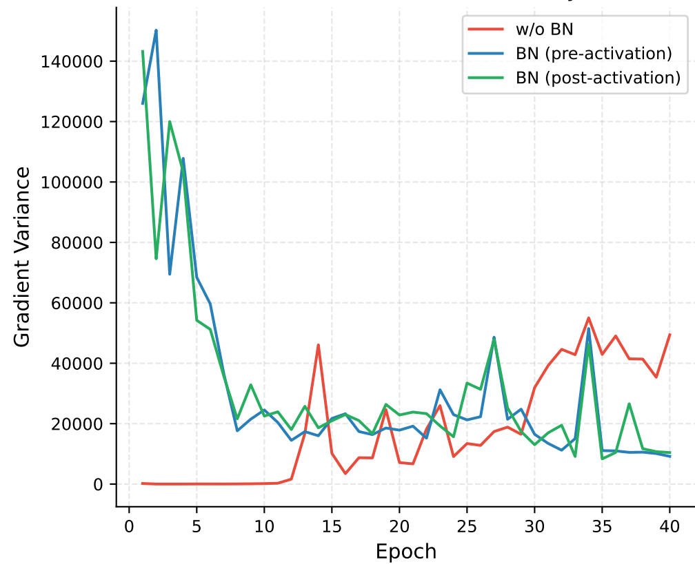
(c) Gradient Variance Evolution (Layer 2)
