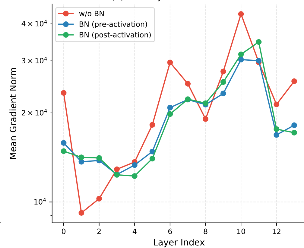
(b) Per-Layer Gradient Norm
