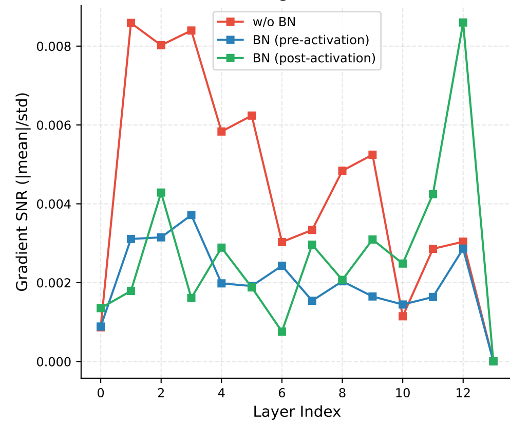
(e) Gradient Signal-to-Noise Ratio
