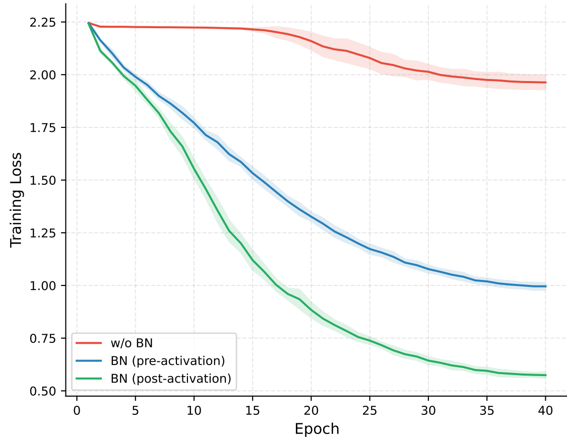
(a) Training Loss Convergence (SVHN_simple_cnn)
