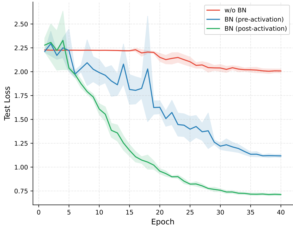
(b) Test Loss Convergence (SVHN_simple_cnn)
