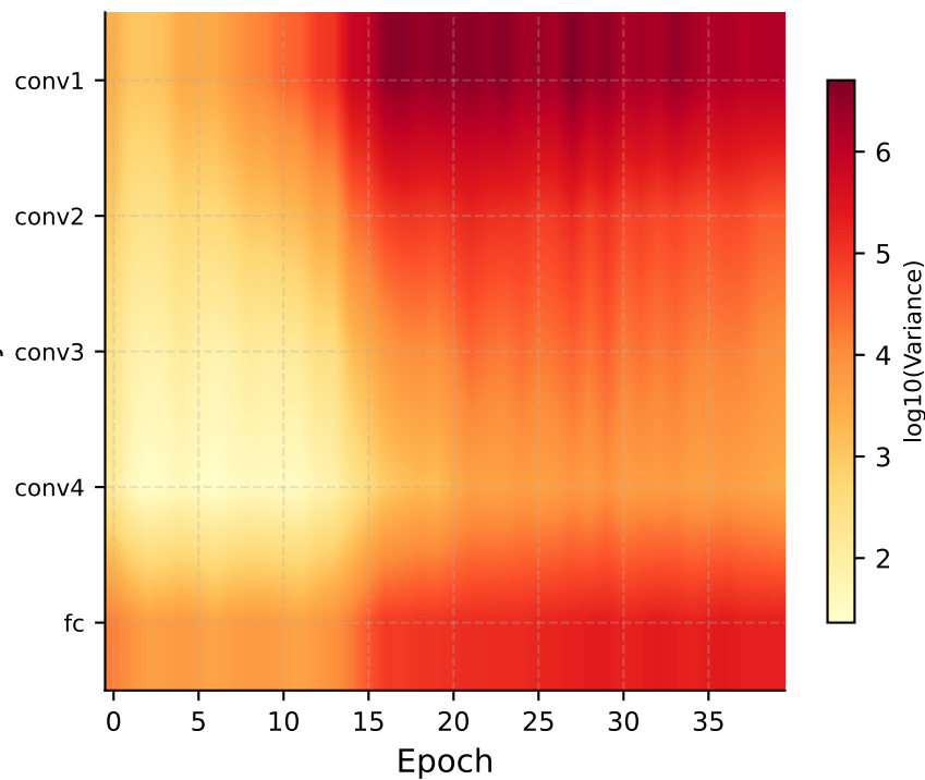
w/o BN
