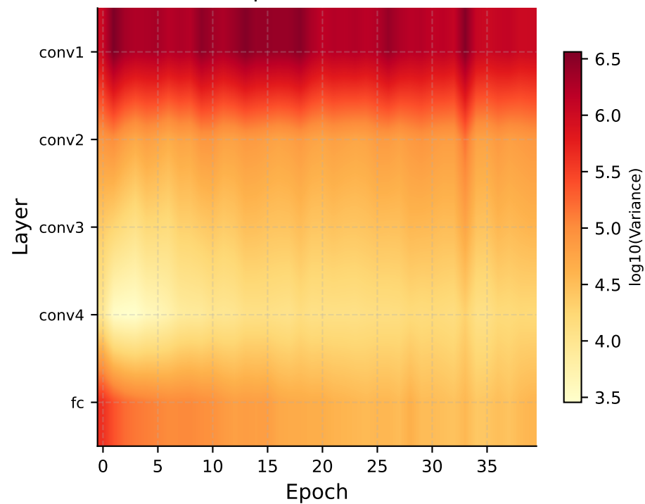
BN (post-activation)
