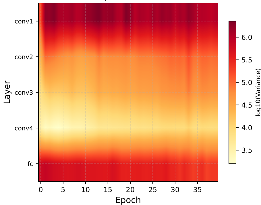
BN (pre-activation)
