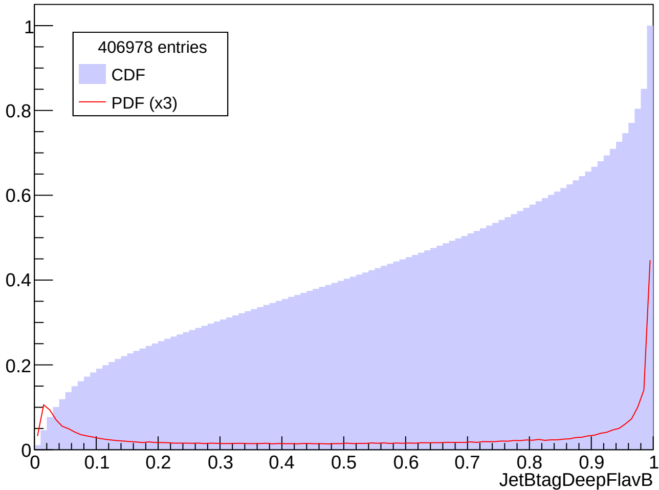
Prob. Distrib. for abs(Eta) in [0.0, 0.5], Pt in [20, 30] GeV
