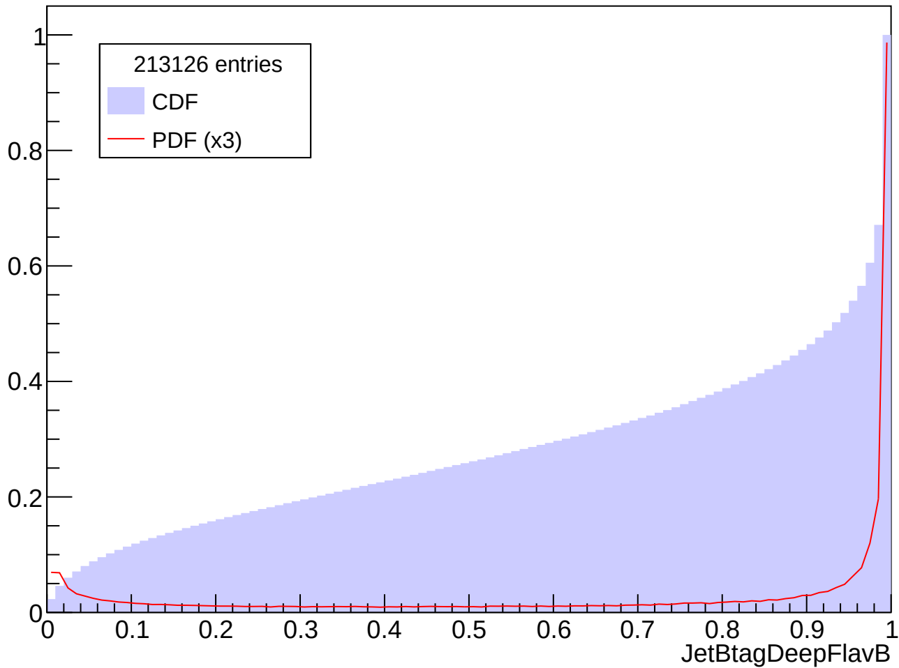
Prob. Distrib. for abs(Eta) in [0.0, 0.5], Pt in [140, 160] GeV
