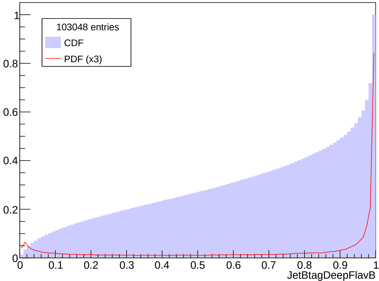
Prob. Distrib. for abs(Eta) in [0.0, 0.5], Pt in [250, 300] GeV
