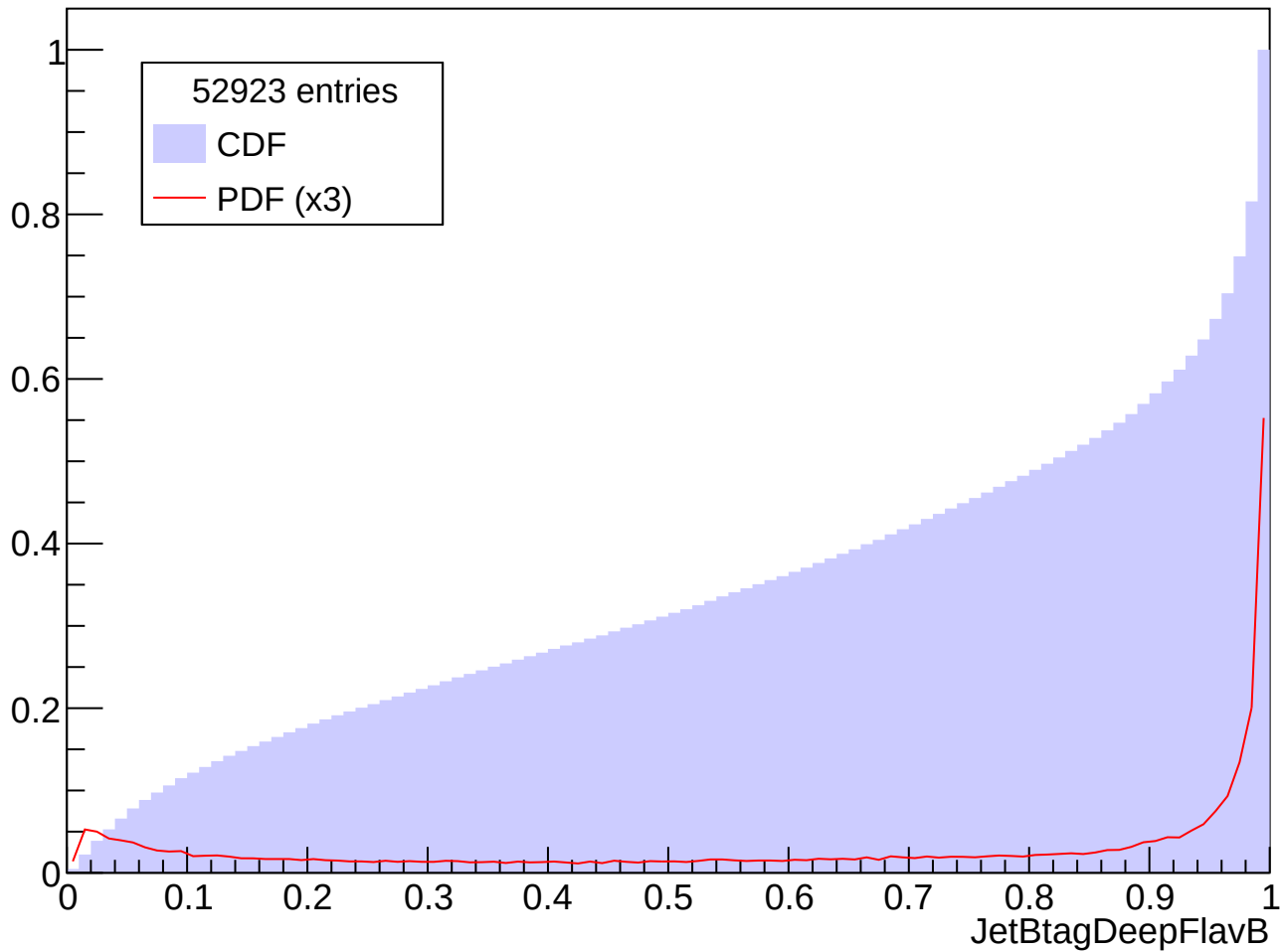
Prob. Distrib. for abs(Eta) in [0.0, 0.5], Pt in [400, 600] GeV
