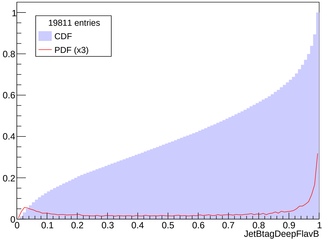
Prob. Distrib. for abs(Eta) in [0.0, 0.5], Pt in [600, 1000] GeV
