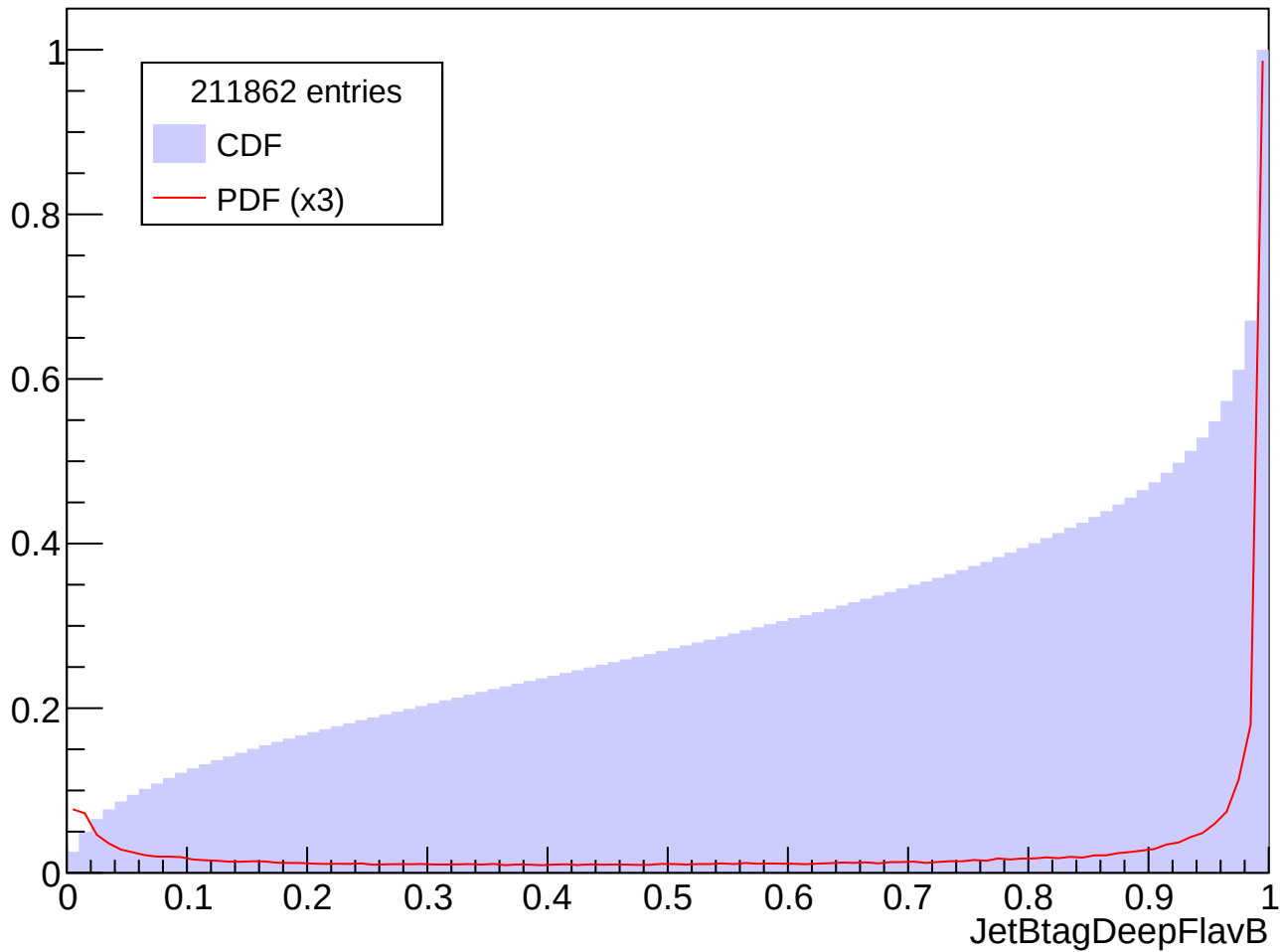
Prob. Distrib. for abs(Eta) in [0.0, 0.5], Pt in [80, 90] GeV
