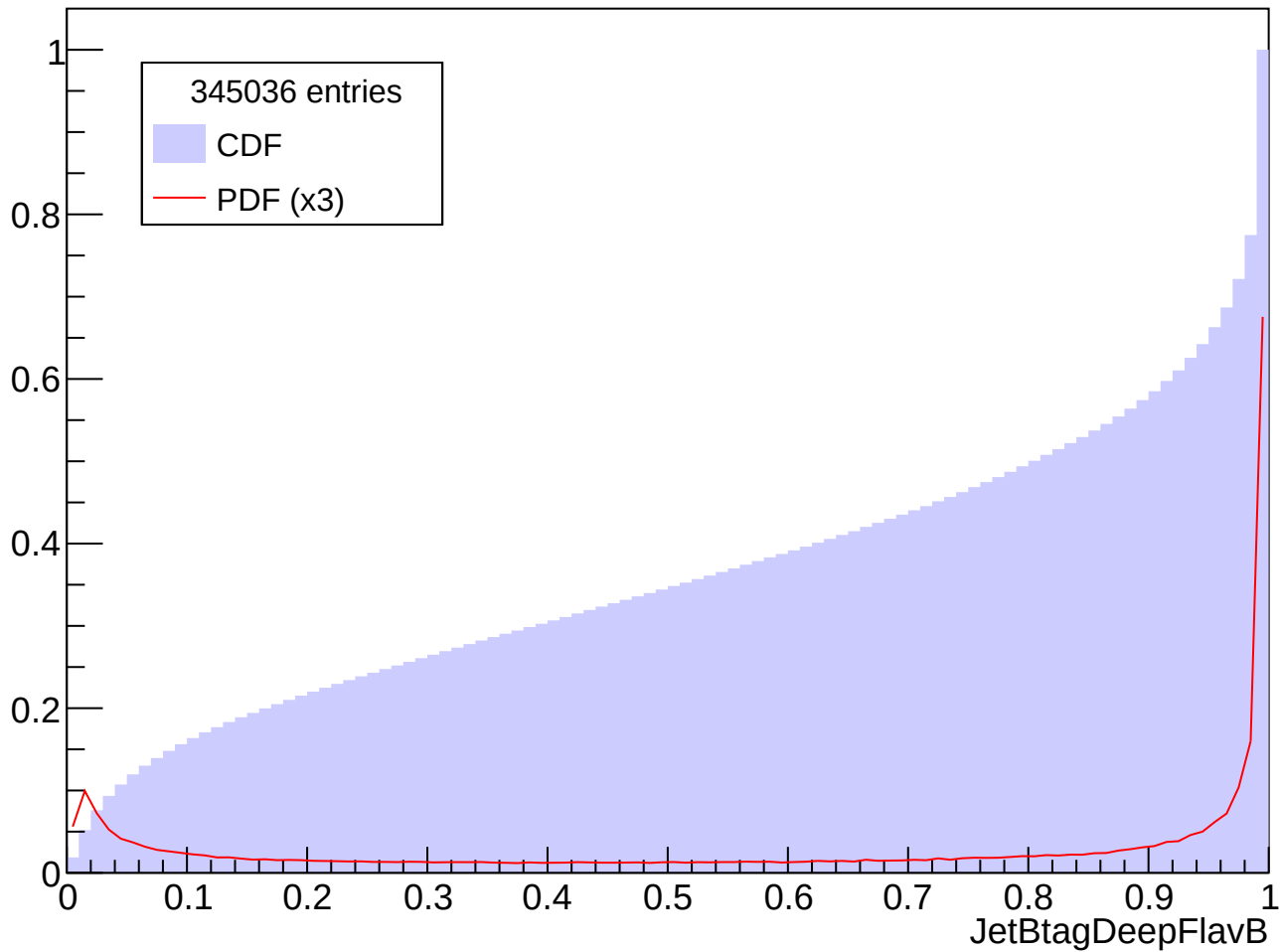
Prob. Distrib. for abs(Eta) in [0.5, 1.0], Pt in [30, 40] GeV
