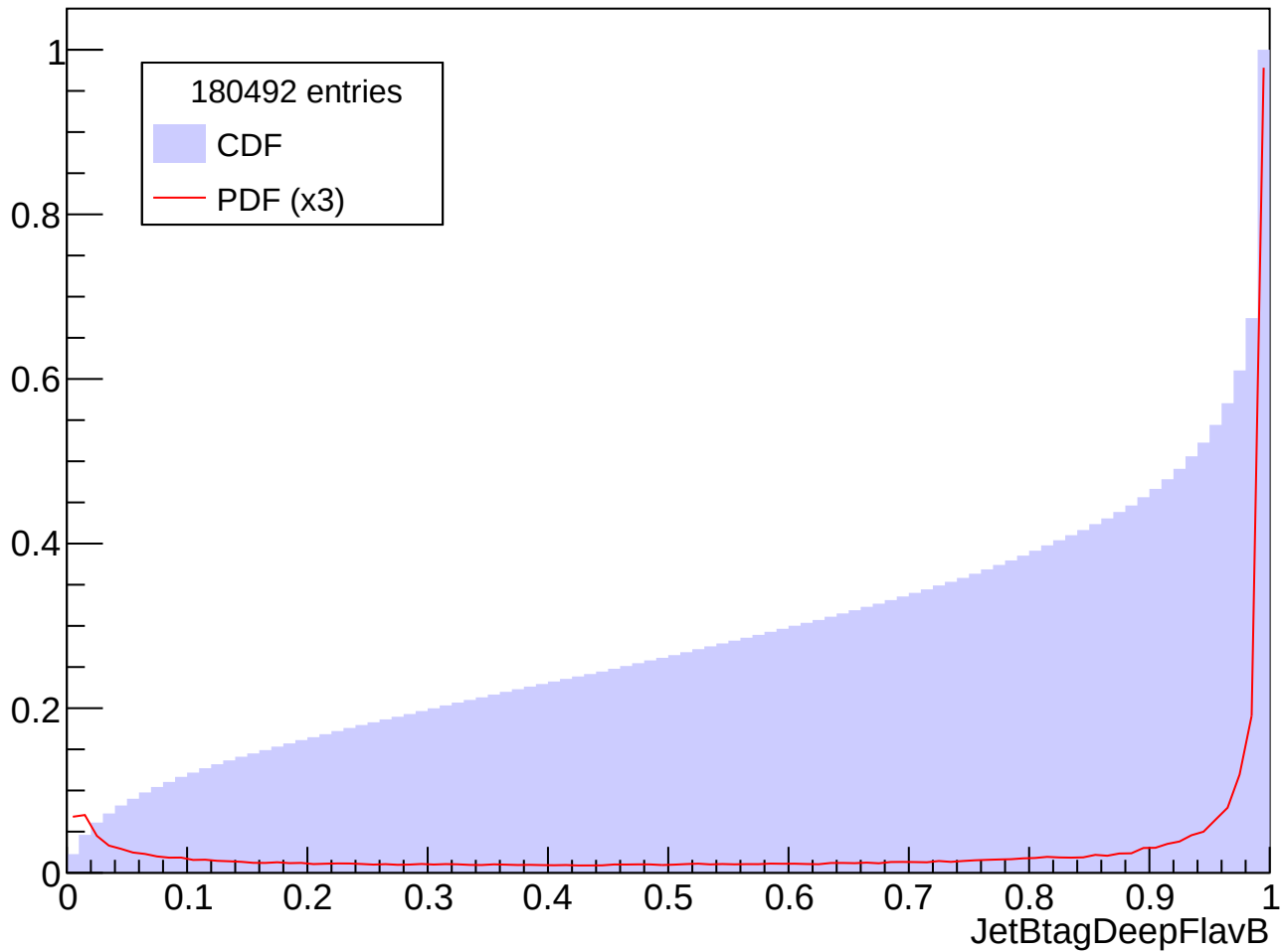
Prob. Distrib. for abs(Eta) in [0.5, 1.0], Pt in [140, 160] GeV
