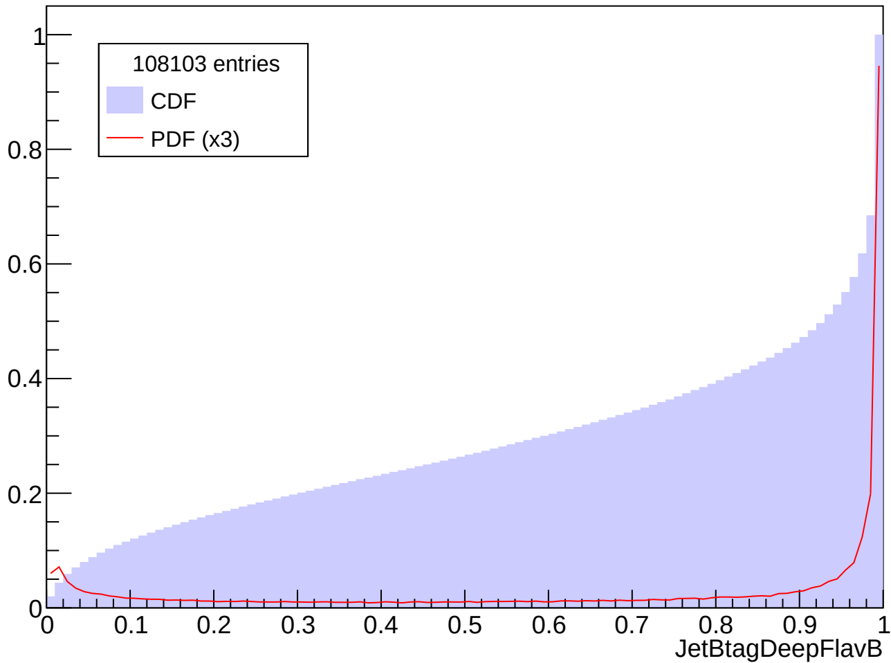
Prob. Distrib. for abs(Eta) in [0.5, 1.0], Pt in [180, 200] GeV
