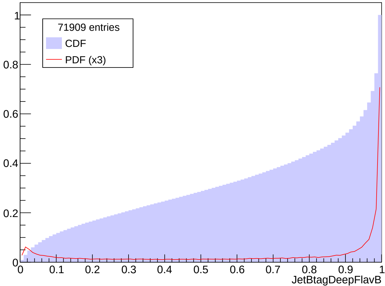
Prob. Distrib. for abs(Eta) in [0.5, 1.0], Pt in [300, 400] GeV
