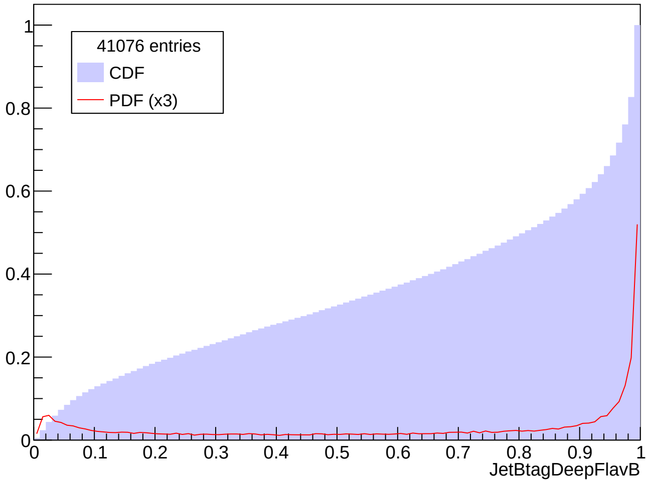
Prob. Distrib. for abs(Eta) in [0.5, 1.0], Pt in [400, 600] GeV
