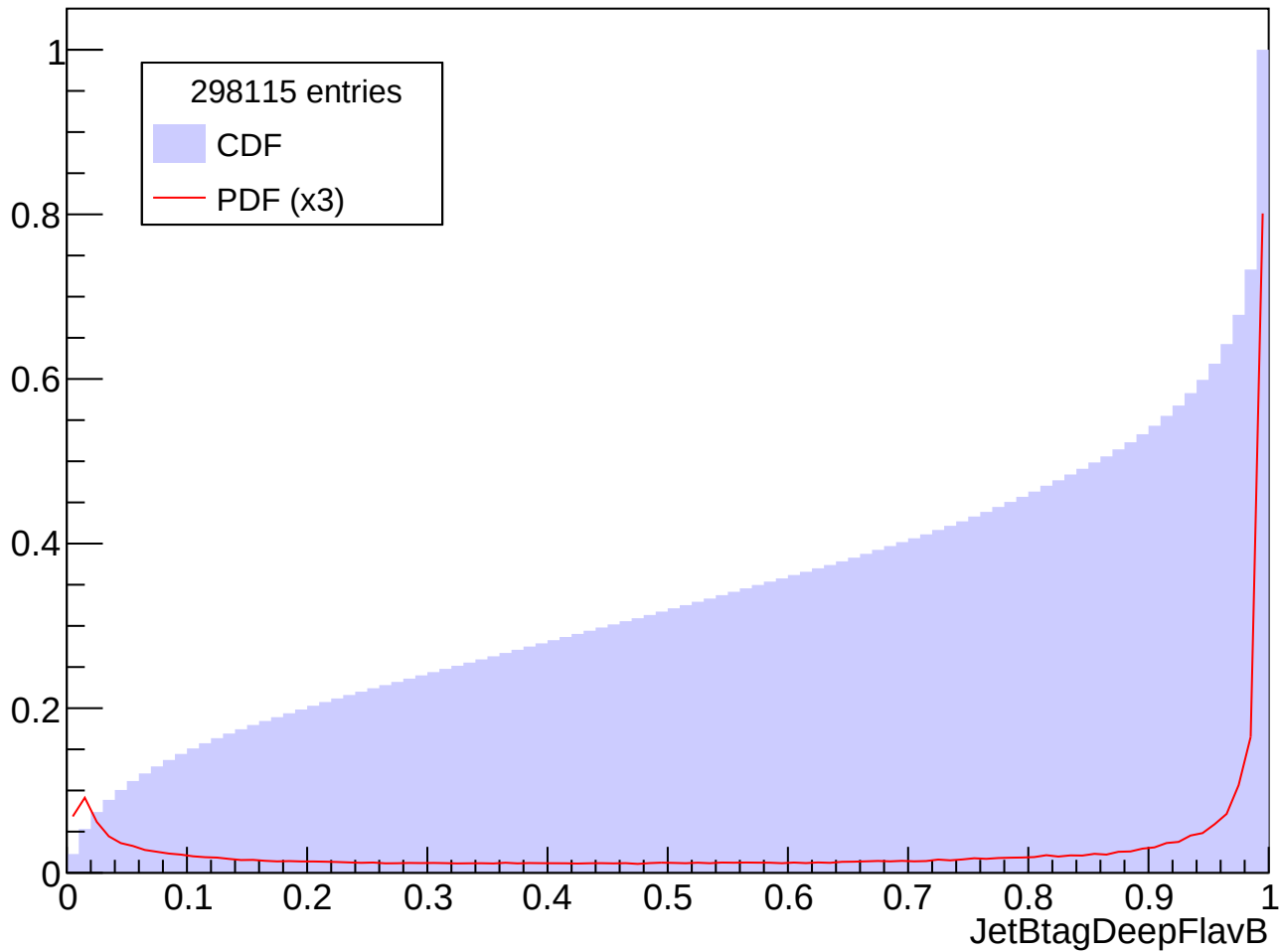
Prob. Distrib. for abs(Eta) in [0.5, 1.0], Pt in [40, 50] GeV
