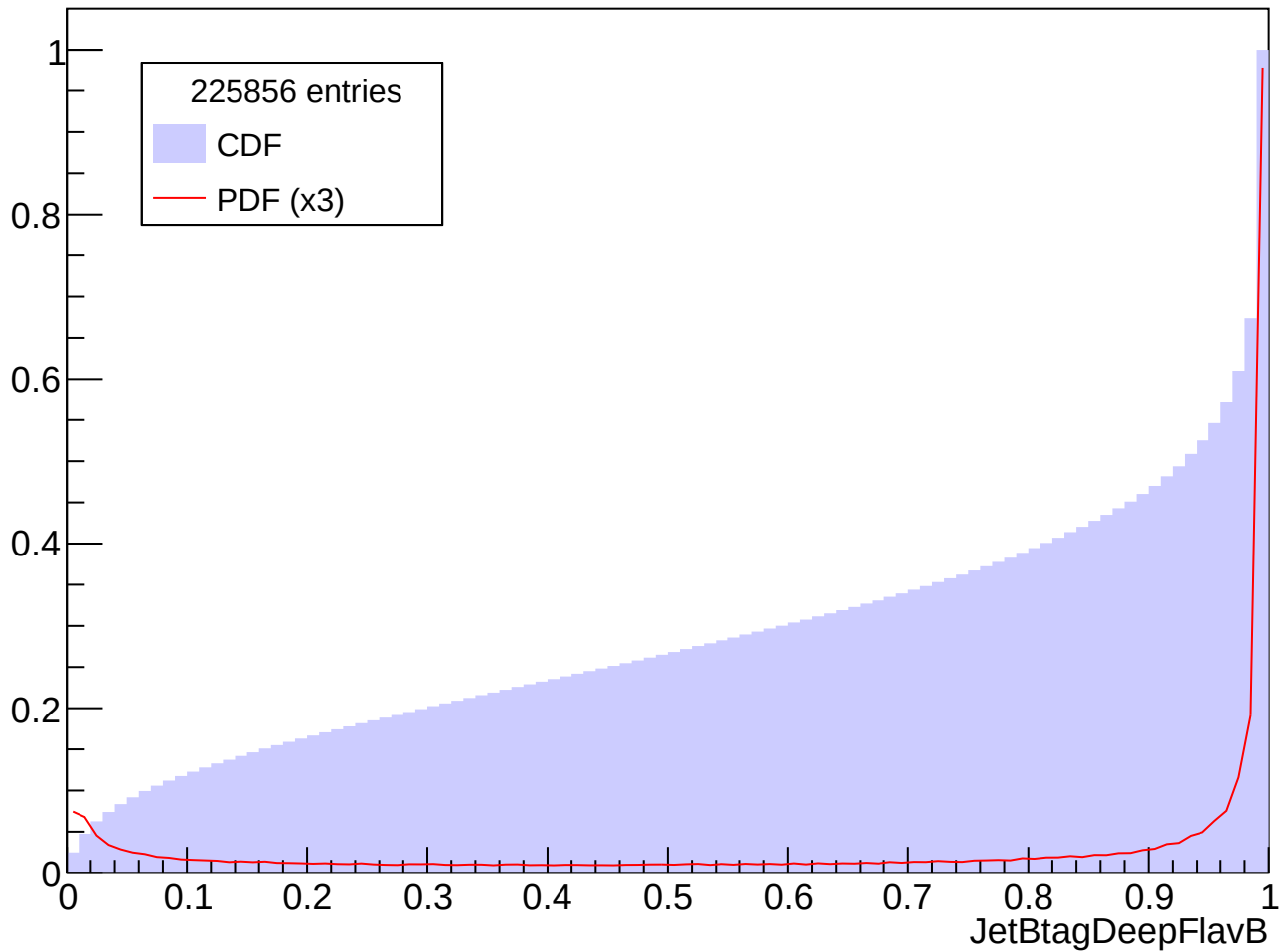
Prob. Distrib. for abs(Eta) in [0.5, 1.0], Pt in [120, 140] GeV
