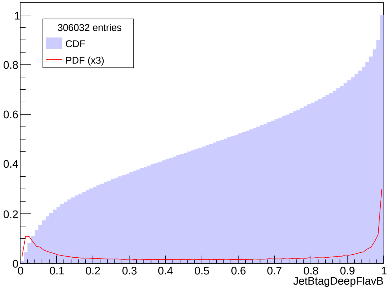
Prob. Distrib. for abs(Eta) in [1.0, 1.5], Pt in [20, 30] GeV
