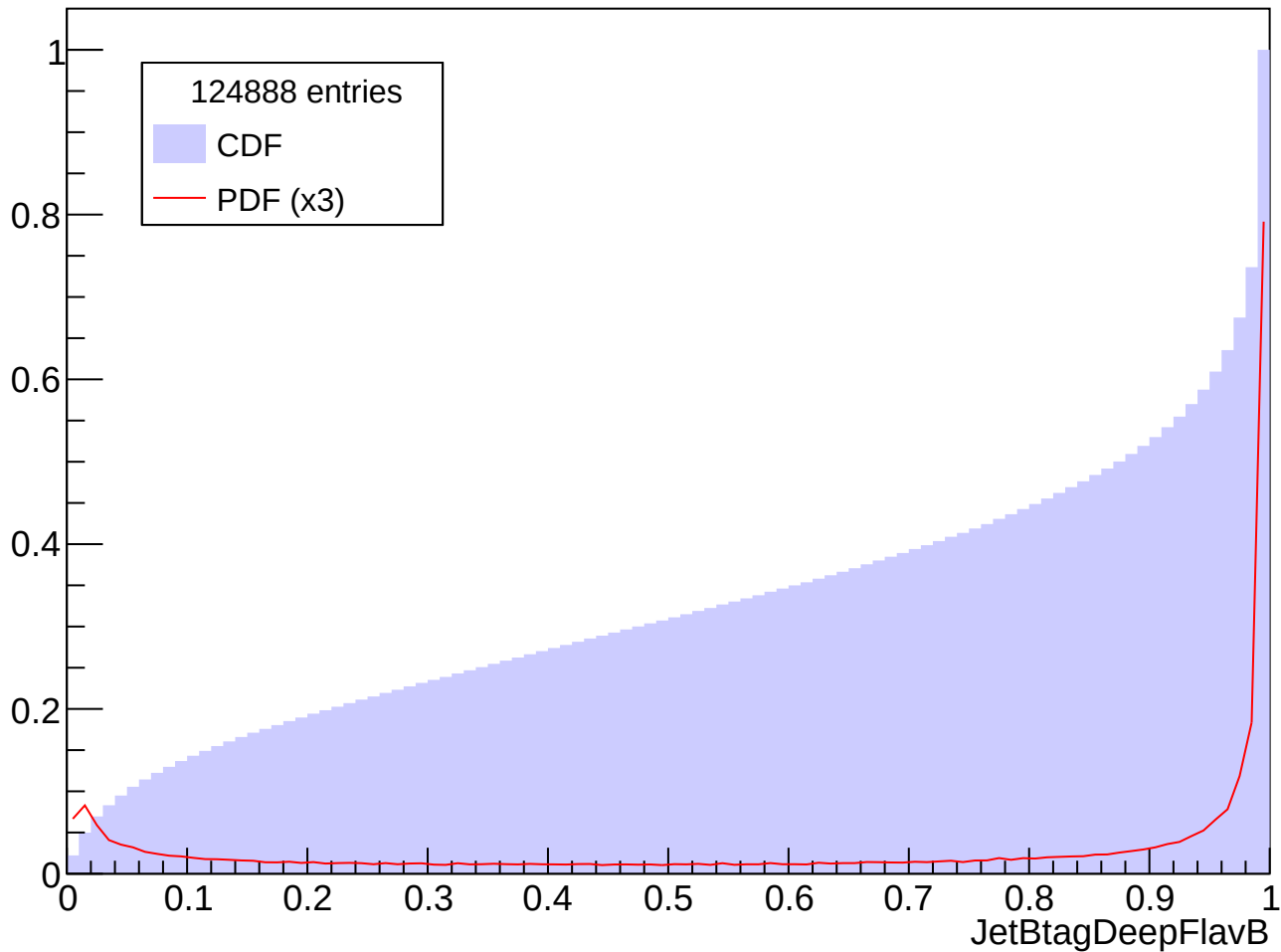
Prob. Distrib. for abs(Eta) in [1.0, 1.5], Pt in [140, 160] GeV
