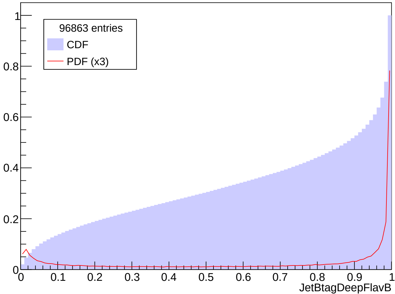
Prob. Distrib. for abs(Eta) in [1.0, 1.5], Pt in [160, 180] GeV
