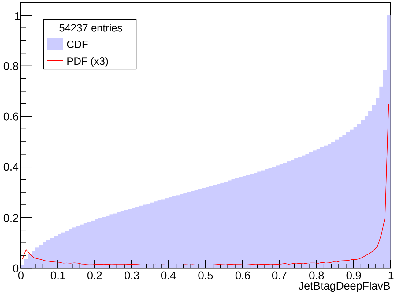
Prob. Distrib. for abs(Eta) in [1.0, 1.5], Pt in [250, 300] GeV
