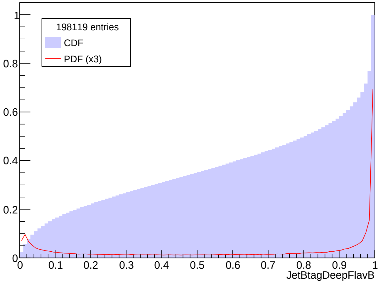
Prob. Distrib. for abs(Eta) in [1.0, 1.5], Pt in [50, 60] GeV
