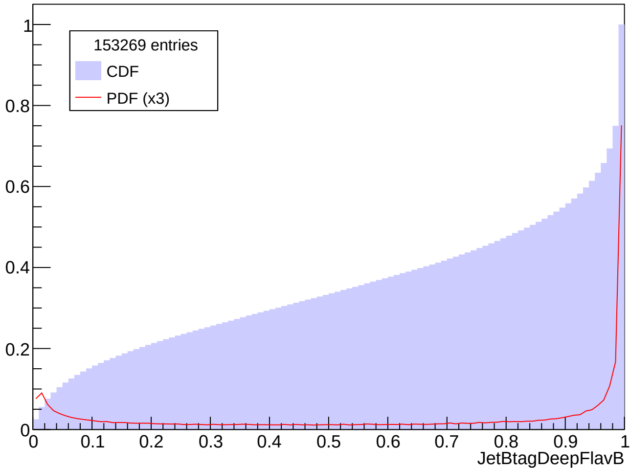
Prob. Distrib. for abs(Eta) in [1.0, 1.5], Pt in [70, 80] GeV
