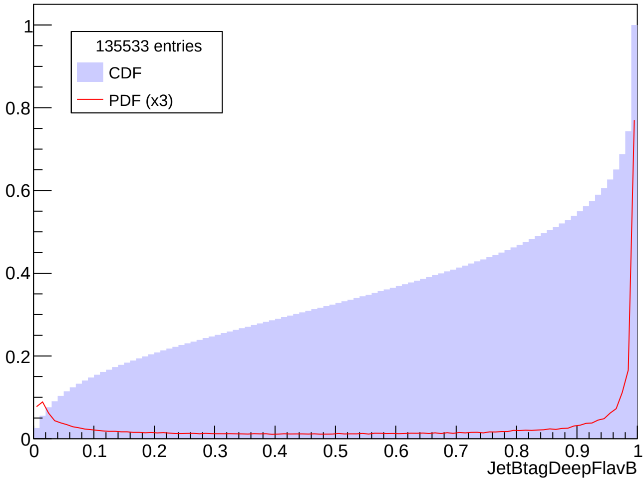
Prob. Distrib. for abs(Eta) in [1.0, 1.5], Pt in [80, 90] GeV
