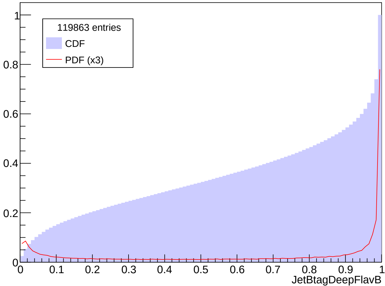
Prob. Distrib. for abs(Eta) in [1.0, 1.5], Pt in [90, 100] GeV
