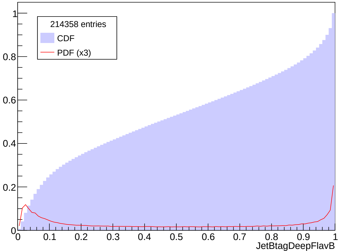
Prob. Distrib. for abs(Eta) in [1.5, 2.0], Pt in [20, 30] GeV
