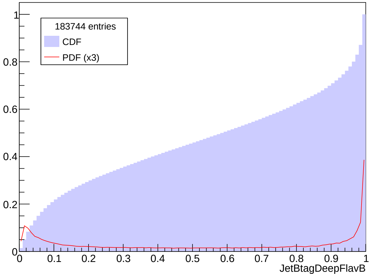
Prob. Distrib. for abs(Eta) in [1.5, 2.0], Pt in [30, 40] GeV
