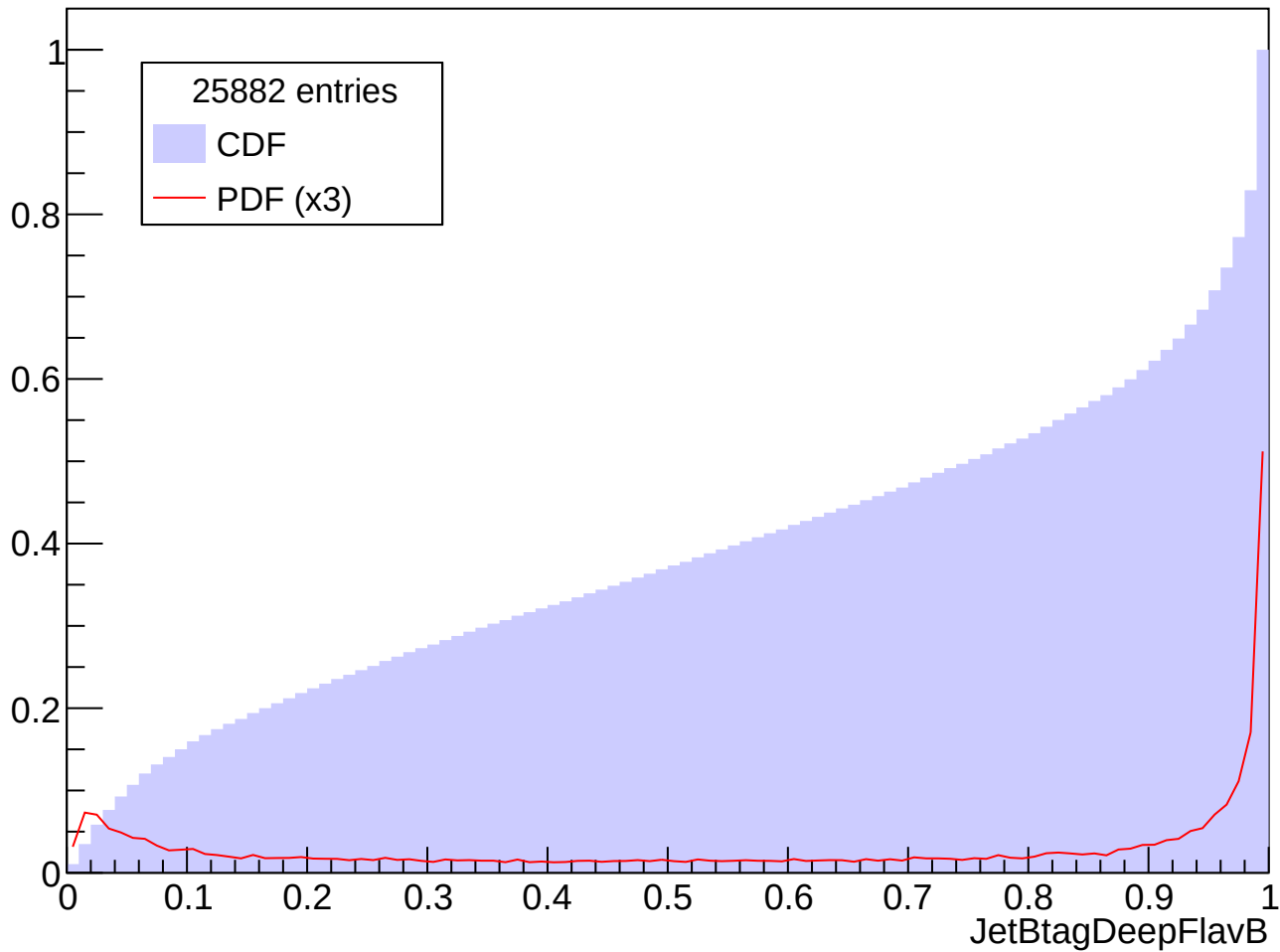
Prob. Distrib. for abs(Eta) in [1.5, 2.0], Pt in [250, 300] GeV
