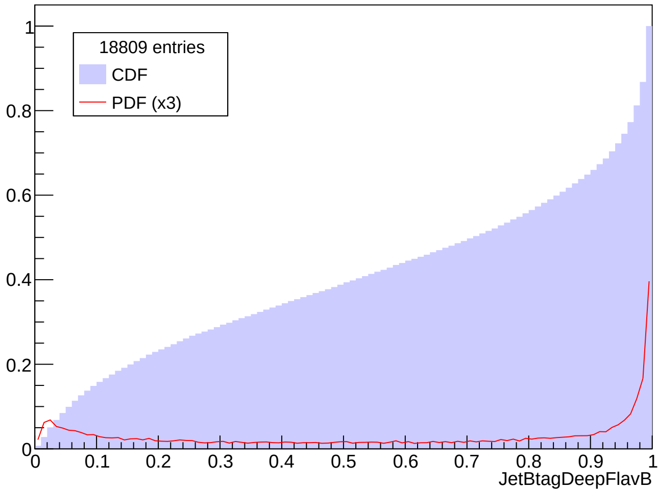
Prob. Distrib. for abs(Eta) in [1.5, 2.0], Pt in [300, 400] GeV
