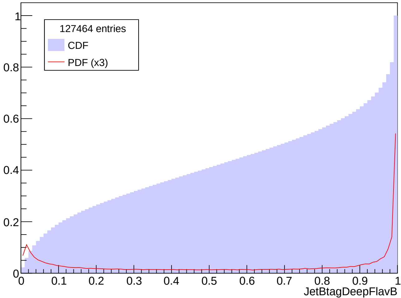
Prob. Distrib. for abs(Eta) in [1.5, 2.0], Pt in [50, 60] GeV
