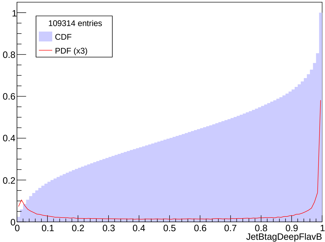
Prob. Distrib. for abs(Eta) in [1.5, 2.0], Pt in [60, 70] GeV
