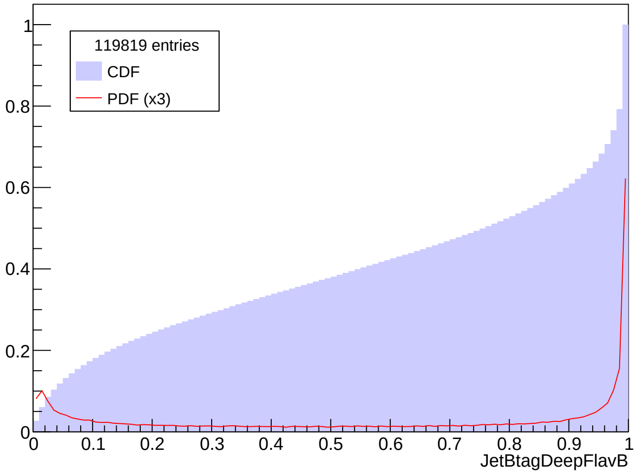
Prob. Distrib. for abs(Eta) in [1.5, 2.0], Pt in [100, 120] GeV
