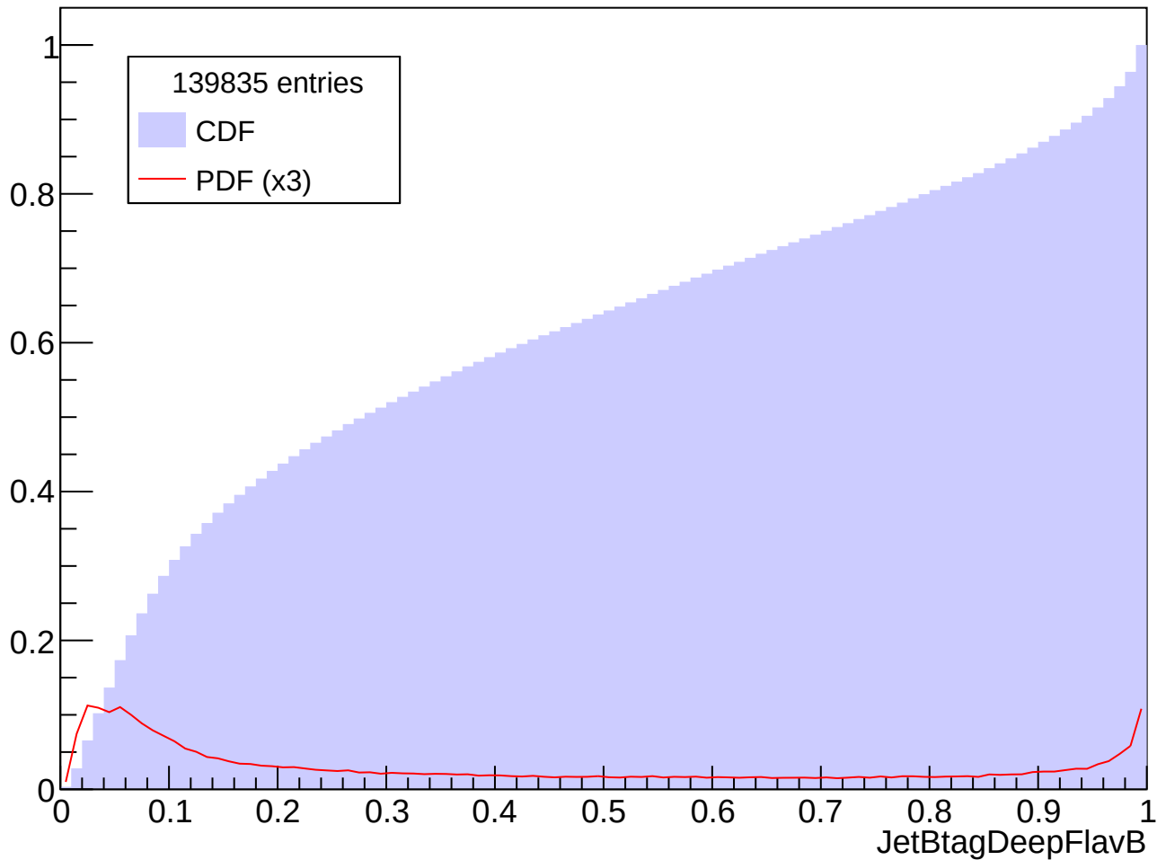
Prob. Distrib. for abs(Eta) in [2.0, 2.5], Pt in [20, 30] GeV
